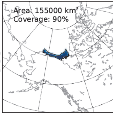
Barrow Sea - continental coast and shelf
