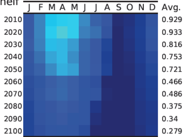
Sea ice thickness
