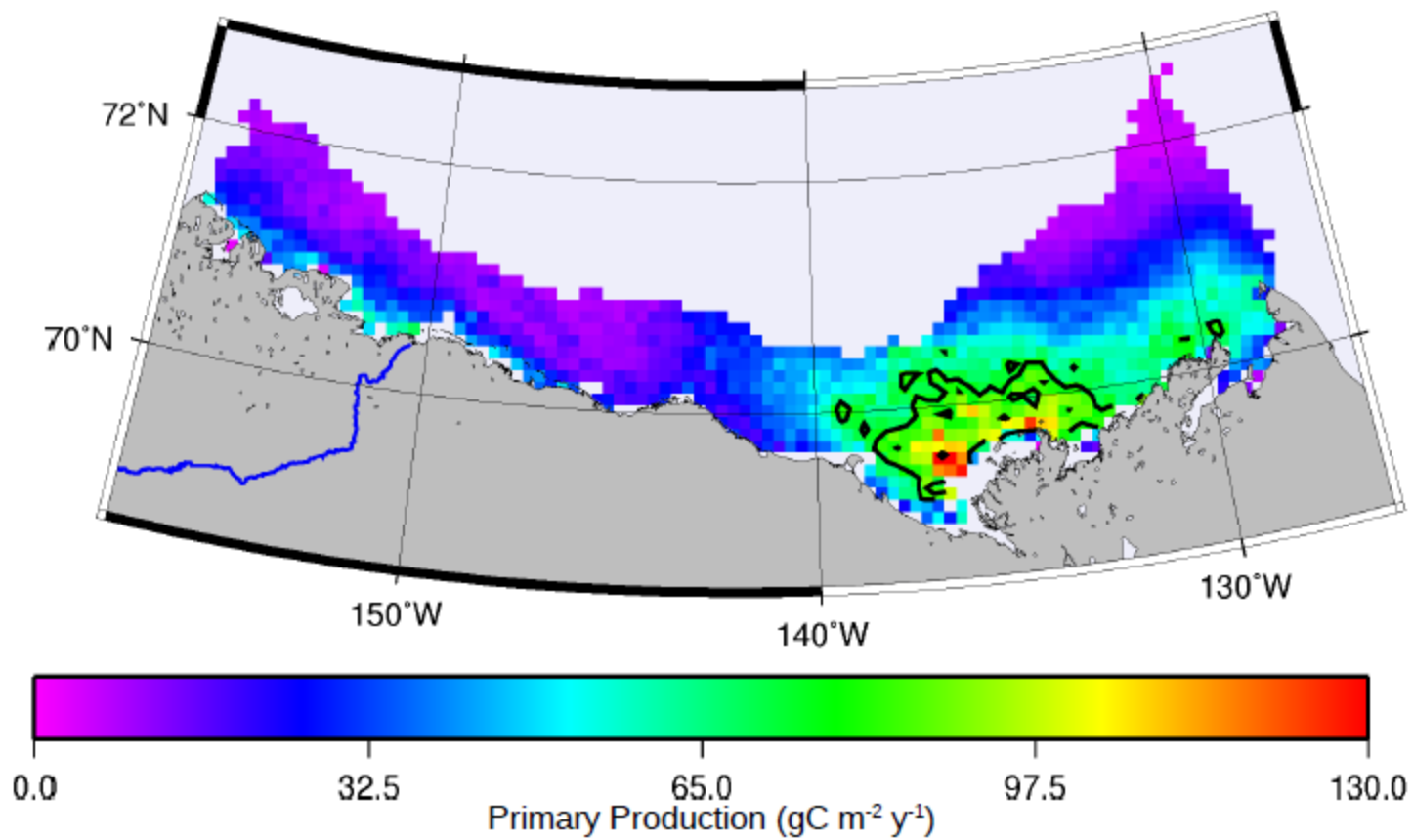
Figure 10: PP production rates of the Beaufort Sea (continental coast and shelf) . Contour lines indicate the 10% most productive pixels based on the 90th percentile analysis (see the method section)
