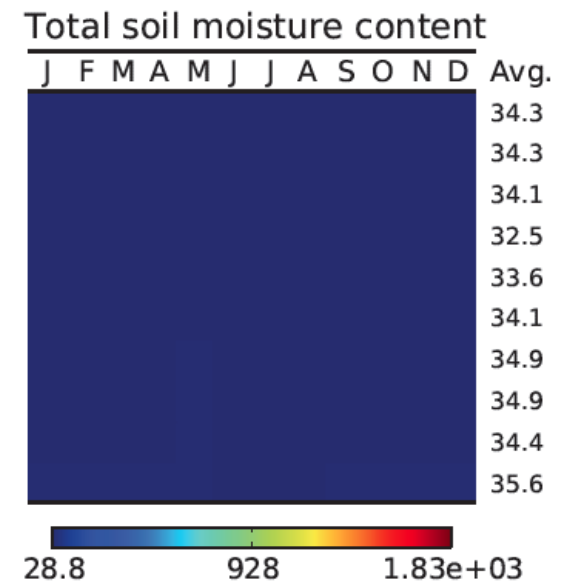
Soil moisture content [kg m -2 ]
