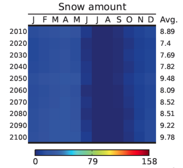
Surface snow amount where land [kg m -2 ]
