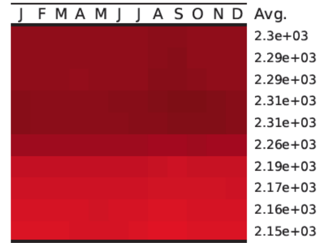
Soil moisture content [kg m -2 ]
