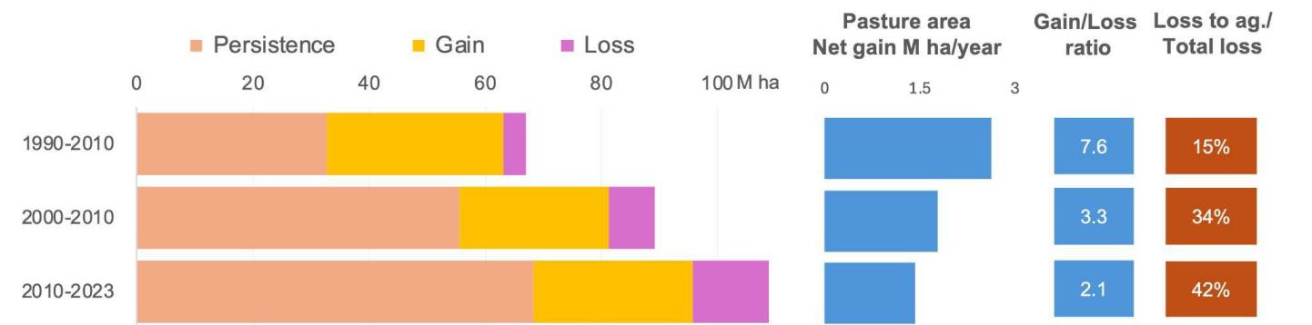
Figure 1. Pasture persistence, gain and loss in the Amazon region from 1990 to 2023
